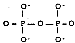
Pyrophosphate
